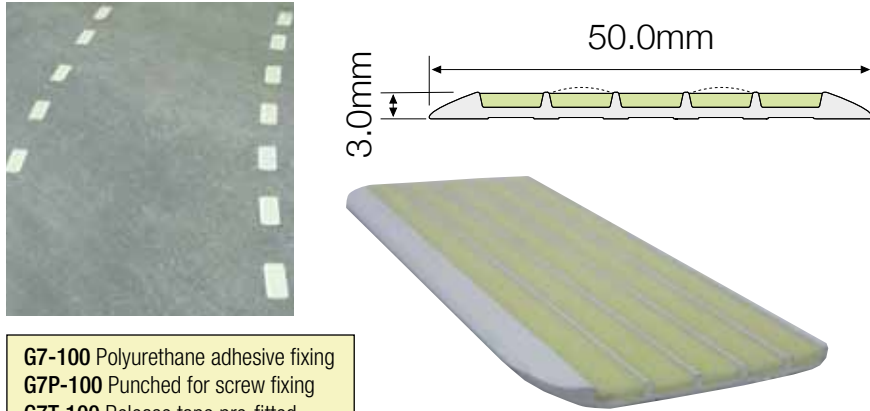
G7-100 Solaris Path Marker Available in 100mm lengths
