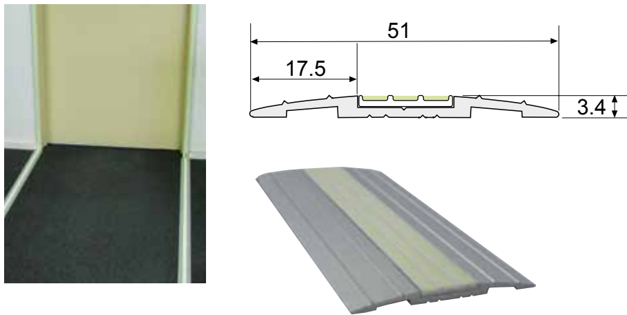
T5-101 Path Marker Available in 1000mm lengths
