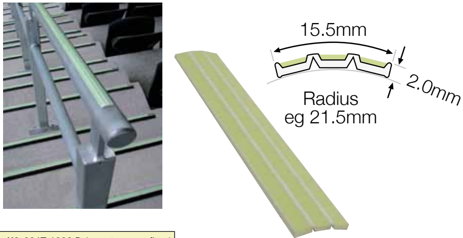
H3-001 Handrail Marker 16mm Available in 1000mm and 1500mm lengths
