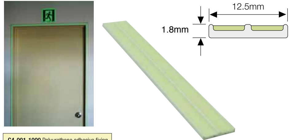
G4-001 Guidance Strip 12.5mm Available in 1000mm lengths
