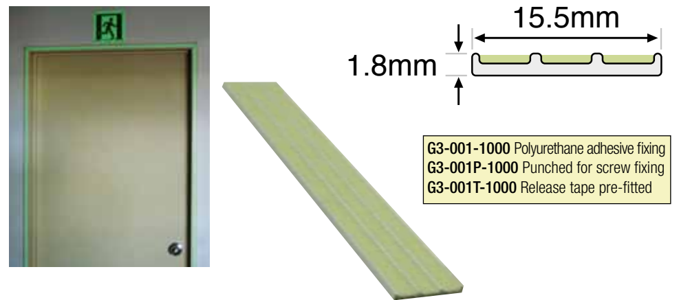
G3-001 Guidance Strip 16mm Available in 1000mm lengths
