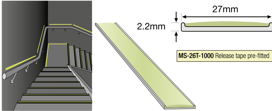
MS-26 Handrail Wall Strip 26mm Available in 1000mm lengths
